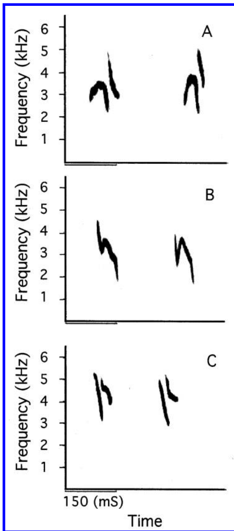
FIGURE 2. Representative flight calls from two individuals of (A) South Hills, (B) call type 2, and (C) call type 5 Red Crossbills. Flight calls of call types differ by the presence of a second element (e.g., call type 2 usually lacks it), frequency (e.g., call type 5 has highest average frequency), and slope of the frequency modulations (e.g., frequency increases in the beginning of the South Hills Crossbill call but not in the others) (Groth 1993; Smith 2005). Figure reproduced from Smith and Benkman (2007).
