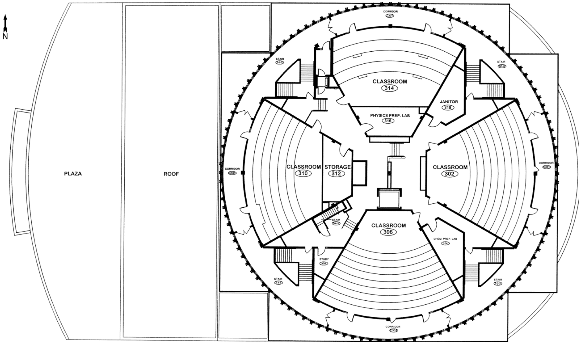
Classroom Building Second Floor
