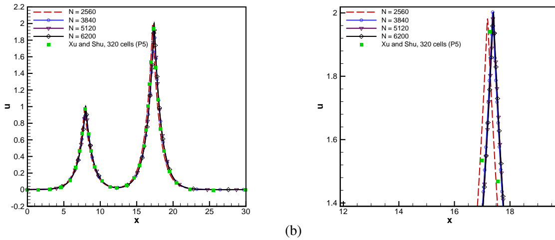
Figure 6.7: (a) Grid refinement study for the initial data (6.16) and (6.17) at the final time t = 18 . (b) Blow-up of the right-hand-side peak.
