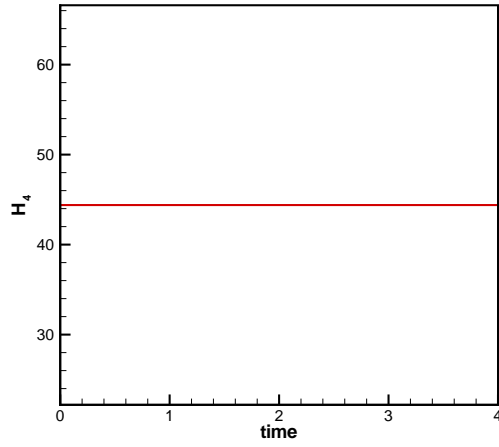
Figure 6.6: The well preserved Hamiltonian H_4 (see Equation (6.11)) by the proposed algorithm. The initial condition is a smooth travelling wave with \kappa = 0 in equation (1.1).
