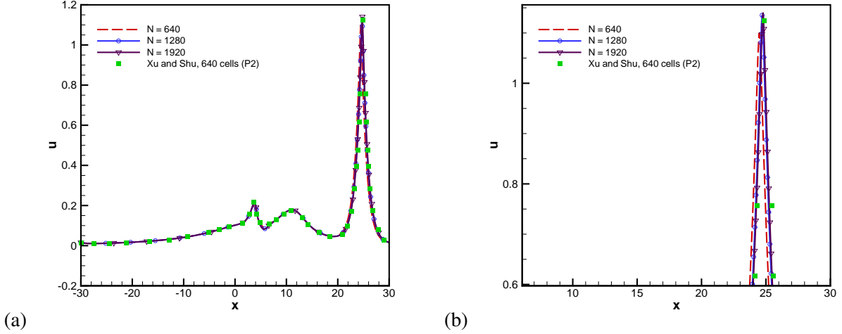
Figure 6.8: (a) Grid refinement study for the initial data (6.18) at t = 20 . (b) Blow-up of the primary peak.
