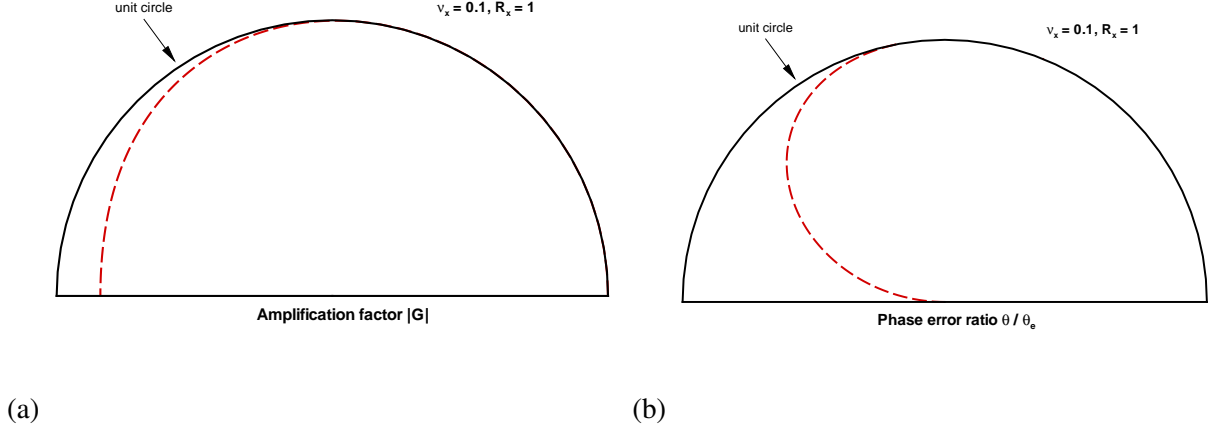
Figure 5.3: Plots of |G| and \mathcal{S} versus \chi_x at v_x = 0.1 and R_x = 1 . Note that the angle \chi_x is from 0 and \pi , counterclockwise. (a) The modulus of amplification factor |G| ; (b) The relative phase-shift error \mathcal{S} . They show that both the amplitude and the phase either have very small errors or have no errors at all before the modified frequency \chi_x reaches \pi/2 .
