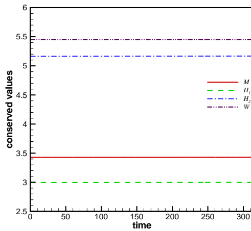
Figure 6.2: Verification of the proposed algorithm. It shows that the quantities M , H_1 , H_2 , and W (see Equations (6.7) and (6.5) ) for the travelling wave problem are well preserved by the proposed algorithm for t > 300 (the time period of 100 cycles, i.e. the initial waveform goes out and in the periodic domain 100 times.)
