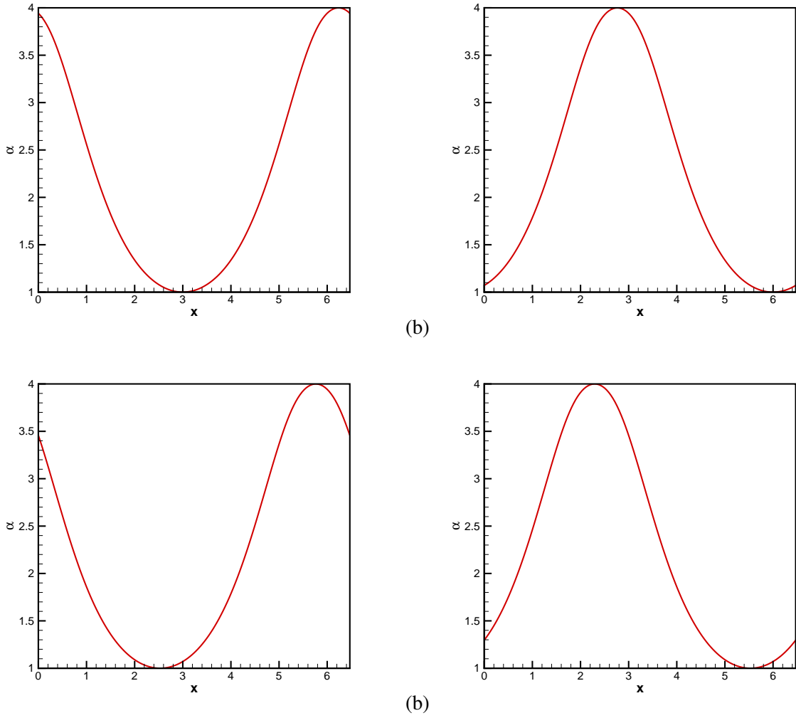
Figure 6.5: Plots of energy density \alpha = u^2 + u_x^2 at different chosen times. (a) t = 1 , (b) t = 2 , (c) t = 3 , and (d) t = 4 . The plots show that \alpha is a periodic function, which indicates the conservation of the Hamiltonian H_1 (see Equation (6.7)).
