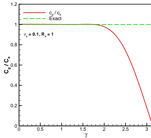
Figure 5.2: Plots of the ratio of group velocity \frac{C_g}{C_e} against the wavenumber \gamma at R_x = 1 and v_x = 0.1 .
