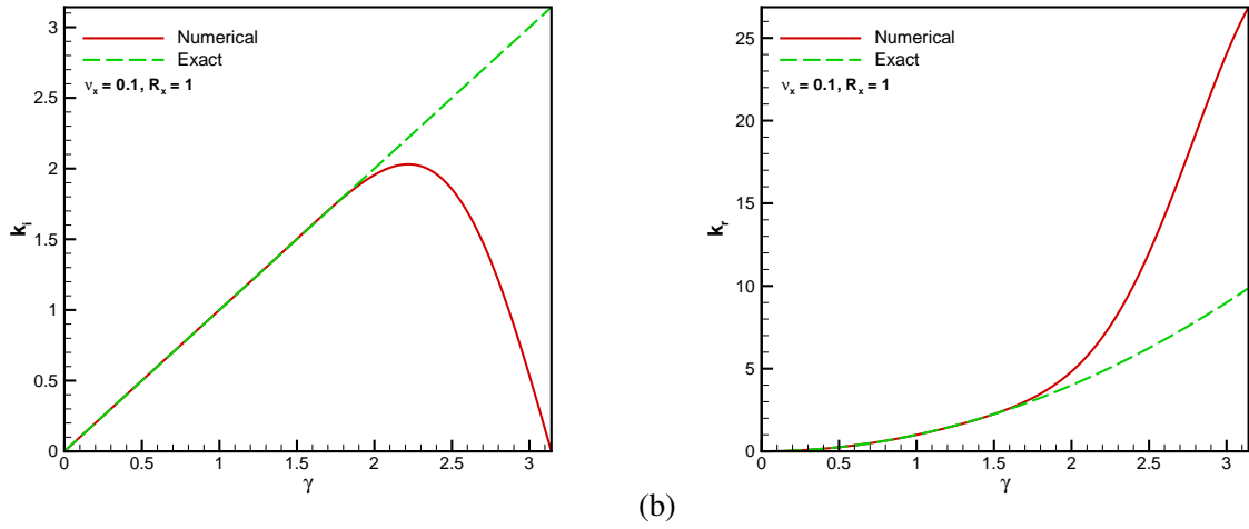
Figure 5.1: The dissipation and phase (dispersion) error analysis. (a) The plot of k_i , the phase error plot. k_i and the modified wavenumber \gamma are visually indistinguishable when \gamma \leq 1.9 . (b) The plot of k_r , the dissipation error plot. k_r and \gamma^2 are visually indistinguishable when \gamma \leq 1.7 .
