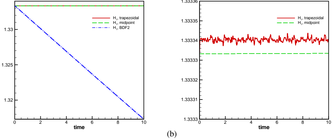
Figure 6.4: Plots of the Hamiltonian values based on grid-independent solutions for the initial data (6.8). \Delta t = \frac{1}{80}\Delta x . (a) The Hamiltonian H_1 (see Equation (6.7)) of three different methods, showing that the midpoint and trapezoidal methods preserve the Hamiltonian, while the second-order BDF method does not. (b) Magnification of the horizontal line in (a). It shows that the Hamiltonian produced by the trapezoidal method has fluctuation.
