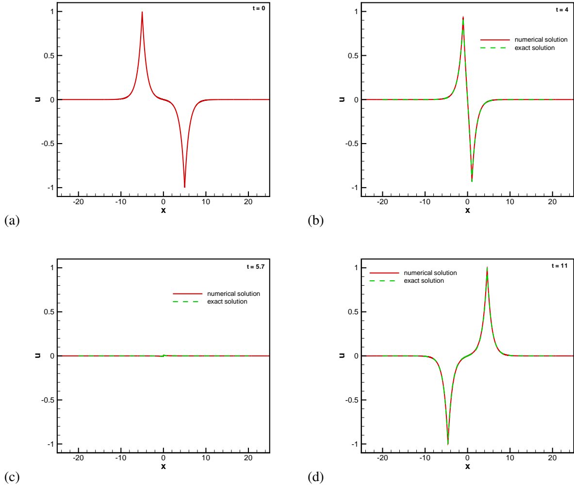
Figure 6.9: The soliton-antisoliton collision: (a) is the initial condition, (b) is the beginning of the collision, (c) is the approximate time of the collision, and (d) is post collision. The theoretical wave speed is c \simeq 0.999977 , and the theoretical collision time is t_c \simeq 5.69327 . The computed solutions are compared with the exact solutions in the Figures. The simulation figures show that the proposed scheme not only accurately captures the wave speed and the collision time, but the numerical solutions are indistinguishable from the exact solutions.
