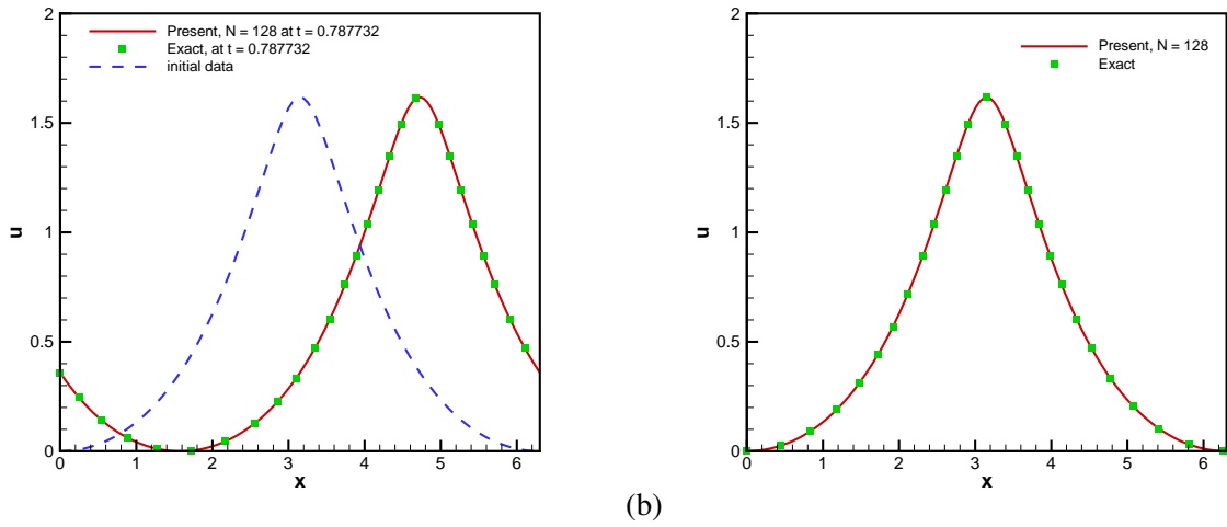
Figure 6.1: The predicted traveling wave solution at (a) t = 0.787732 , (b) t = 3.1509 (over one period). The numerical solutions are compared with the exact solutions that are plotted using square boxes in the illustrations.
