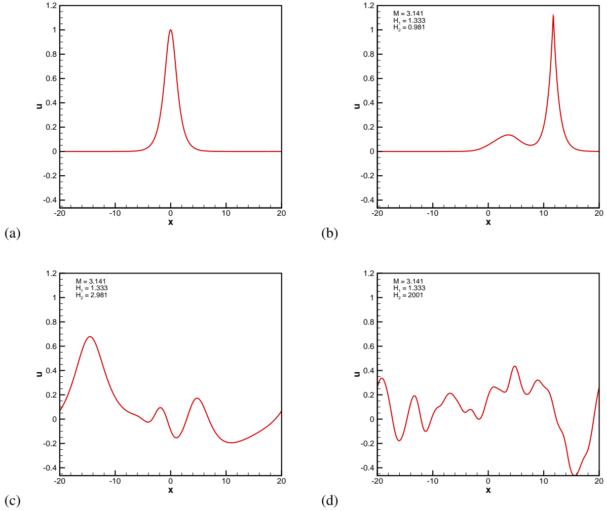
Figure 6.3: The numerical solutions with different values of \kappa at the final time t = 10 . The initial data embedded in a large periodic domain are non-periodic (6.8). The figures show that the solution becomes more dispersive when \kappa increases. (a) Initial condition; (b) \kappa = 10^{-3} ; (c) \kappa = 1 ; (d) \kappa = 10^3 .
