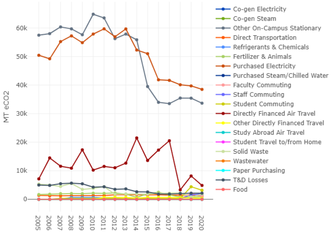
Figure 4: Trends in GHG sources since FY 2005.
