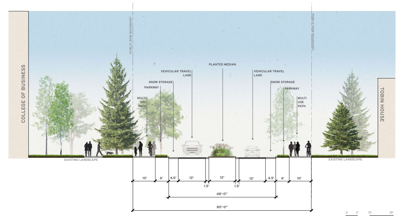
Street Cross Section
