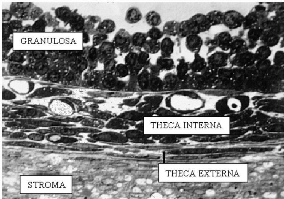
Figure 4-13. Photomicrograph illustrating the three layers of a differentiated follicle.
