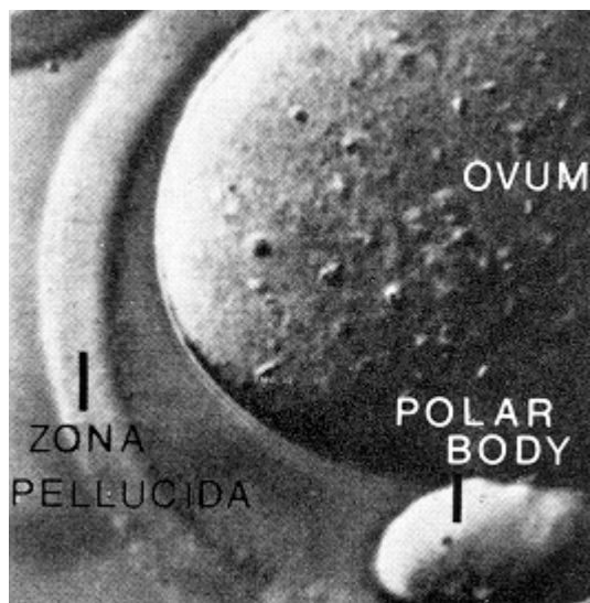
Figure 4-57. A polar body (first) is extruded from the primary oocyte at the completion of meiosis I.
