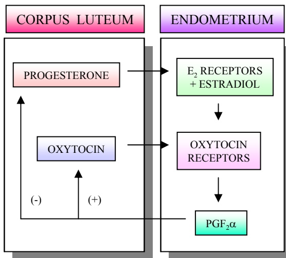
Figure 4-66. Proposed model for regulation of uterine production of \text{PGF}_2\alpha in the sheep.
