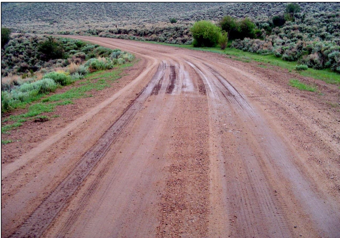
7 – Good 40 - 45 mph Significant roughness, distresses and loose aggregate.
