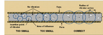
A vibrator's radius of action varies, depending on the vibrator's frequency and head size and the stiffness of the concrete mix. Make sure the vibrator head is large enough and the intervals between vibrator insertions are close enough to vibrate all the concrete.
