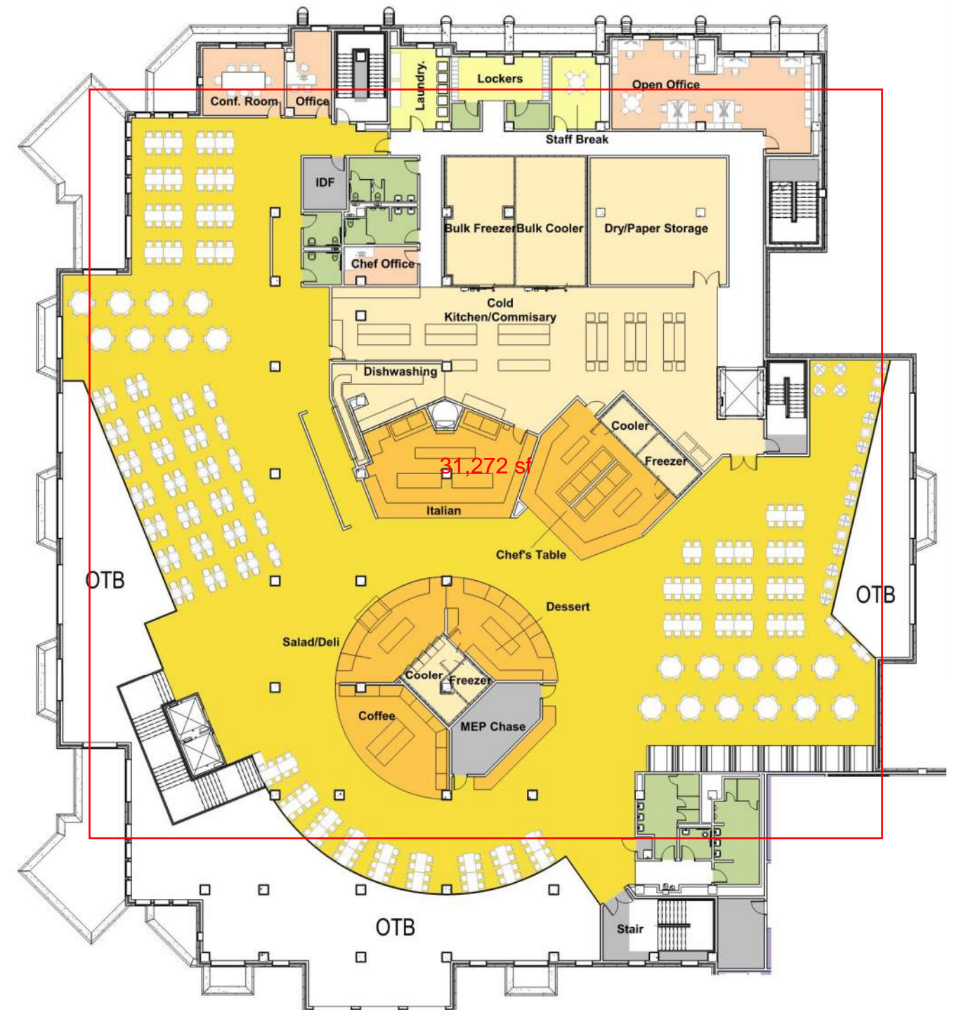
Enlarged Mezzanine Floor Plan – Dining
