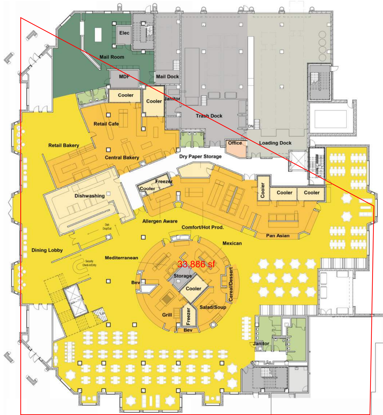
Enlarged First Floor Plan – Dining
