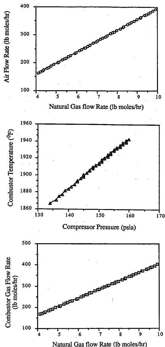
Fig. 6. Sensitivity analysis results.
