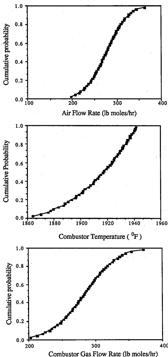
Fig. 5. Probabilistic output results
