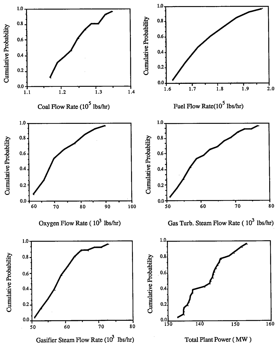
Fig. 7. Probabilistic output results for KRW IGCC flowsheet.
