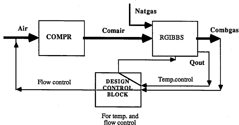
Fig. 3. Process flowsheets for a simple system.
