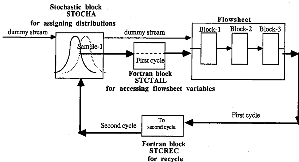
Fig. 1. Basic operation of the stochastic simulation method.
