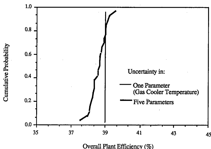
Fig. 8. Uncertainty in overall plant efficiency.
