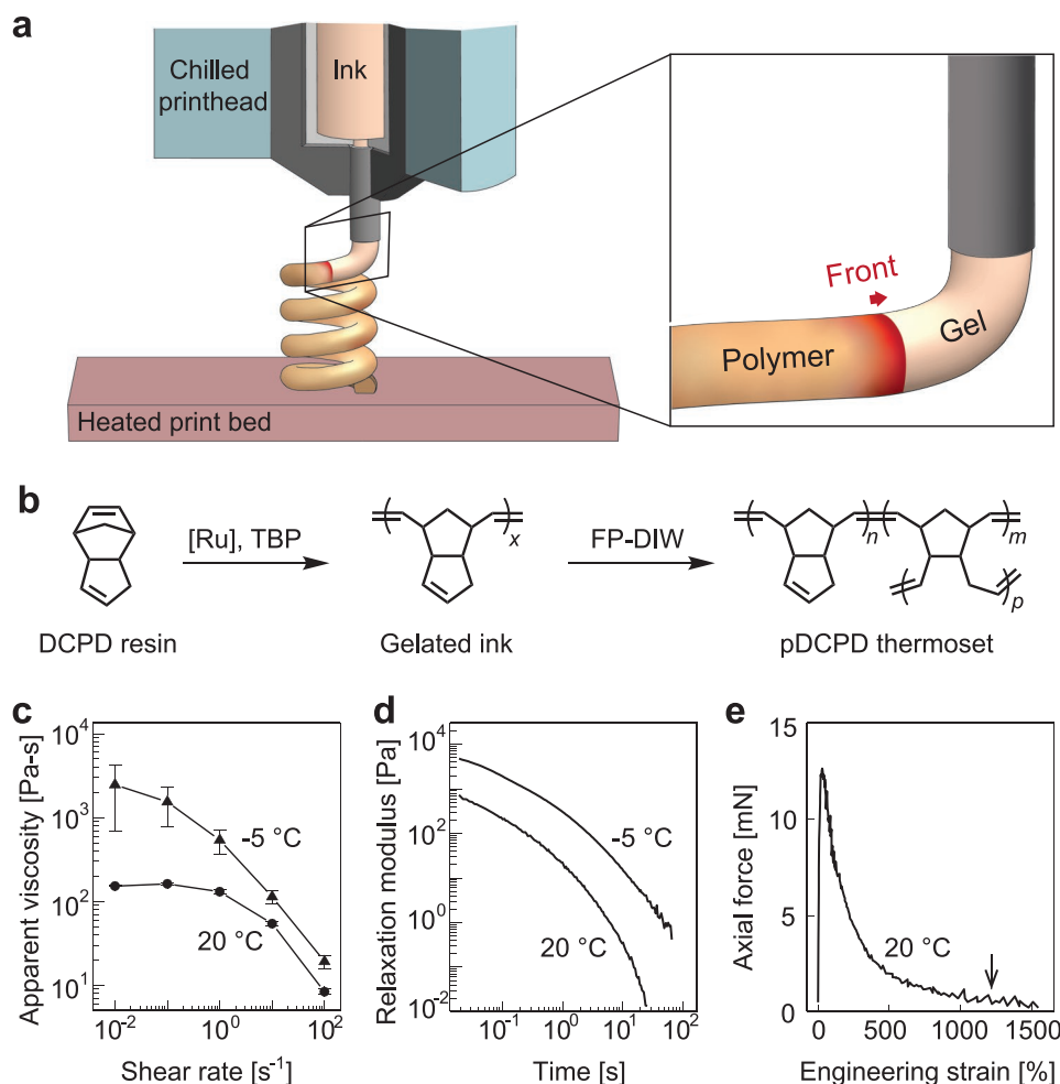
Figure 1. Frontal-polymerization-enabled DIW process for thermoset polymers. a) Schematic of cure front propagation during extrusion of gelled ink from the chilled printhead (−5 °C). The heated print bed (≈100 °C) initiates a self-propagating front, enabling the printing of complex structures. b) Chemical scheme for gelation of DCPD monomer into a printable ink and the frontal polymerization during DIW. c–e) Key rheological properties for printing ink include c) shear-thinning flow, d) a moderate relaxation behavior, and e) a high extensile failure strain (failure is indicated by the arrow).
