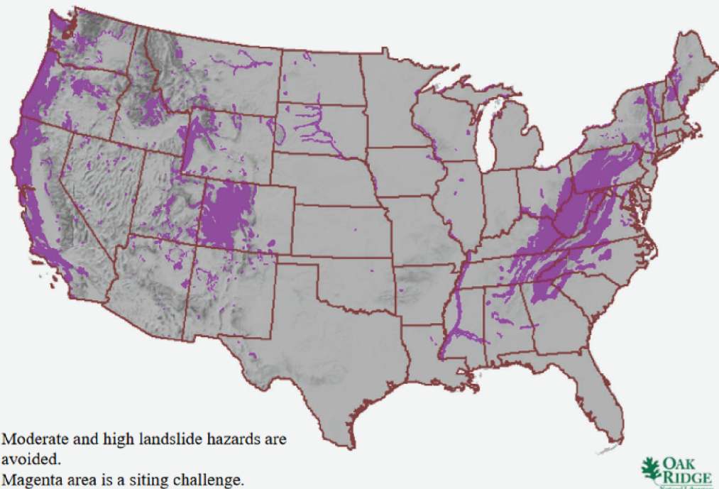
Figure 10: Nominal, bounding SMR landslide- hazards SSEC layer.
