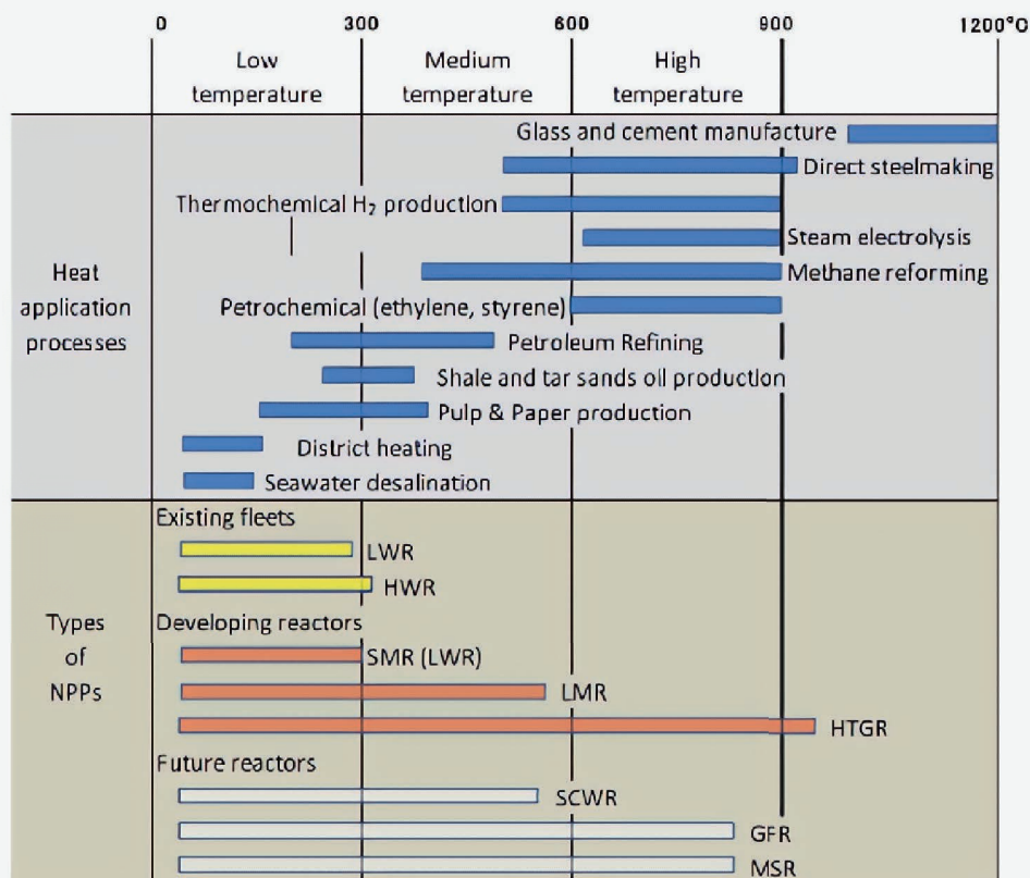
Figure 1 Industrial Temperature Requirements and Nuclear Produced Heat by Reactor Type (International Atomic Energy Agency, 2017) 11
