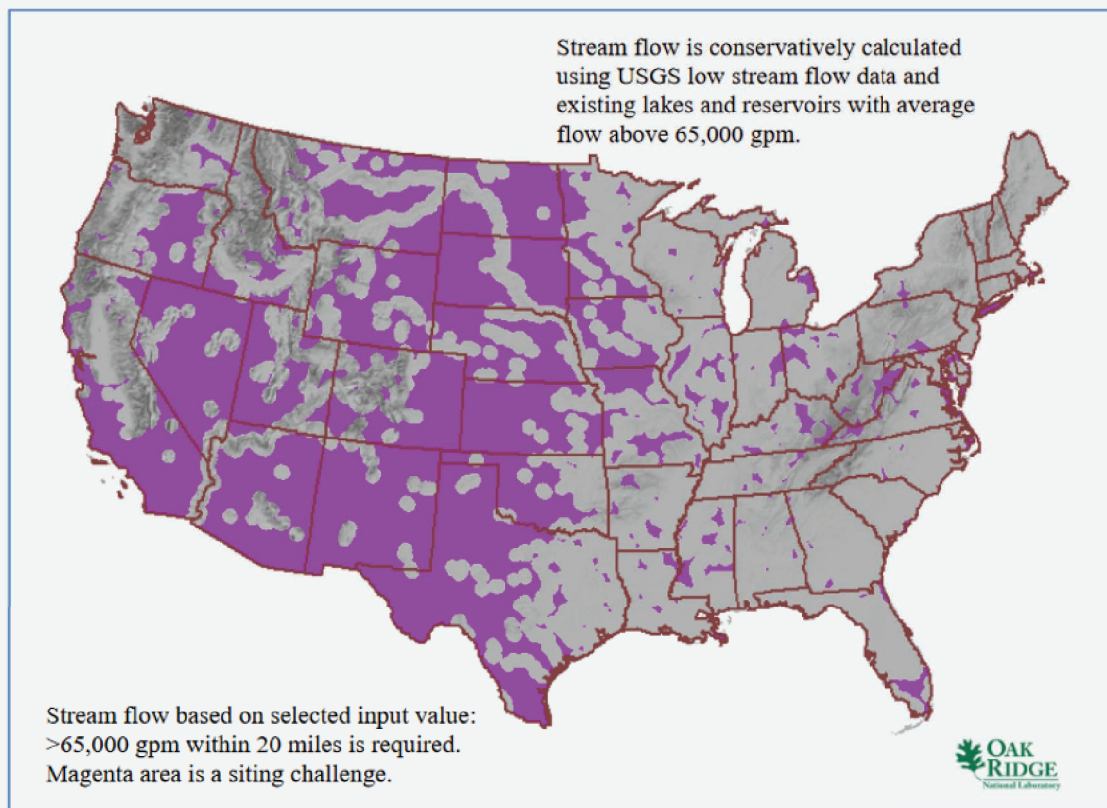
Figure 13: Nominal, bounding SMR minimum low-stream- flow SSEC layer.
