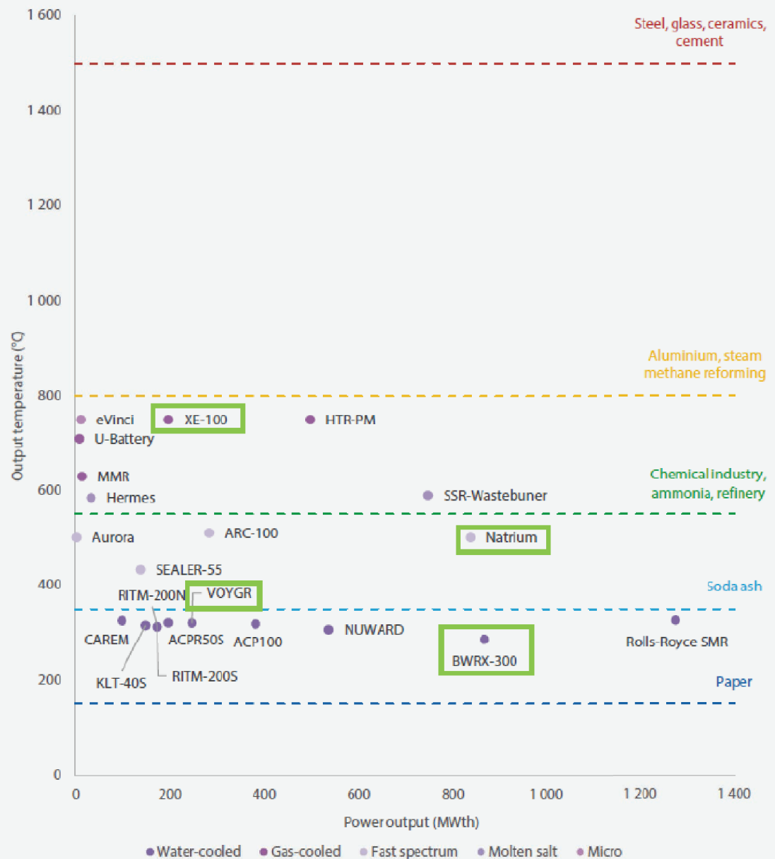
Figure 11: Market Application of SMR designs (Coffey, 2023).
