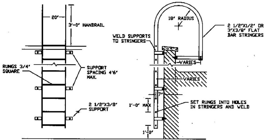
STANDARD ROOF LADDER DETAIL
