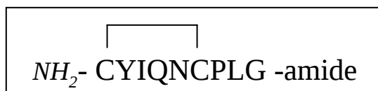
Figure 2-11. Structure of oxytocin.
