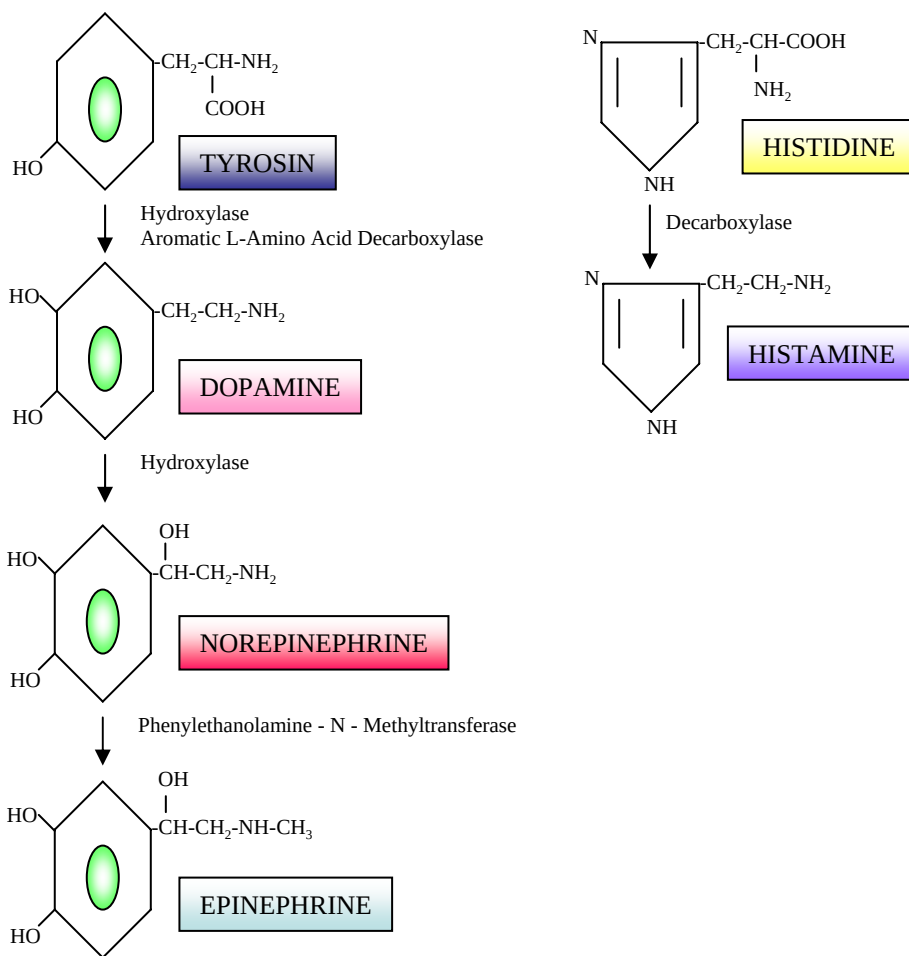
Figure 2-24. Synthesis of catecholamines and histamine from amino acid precursors.
