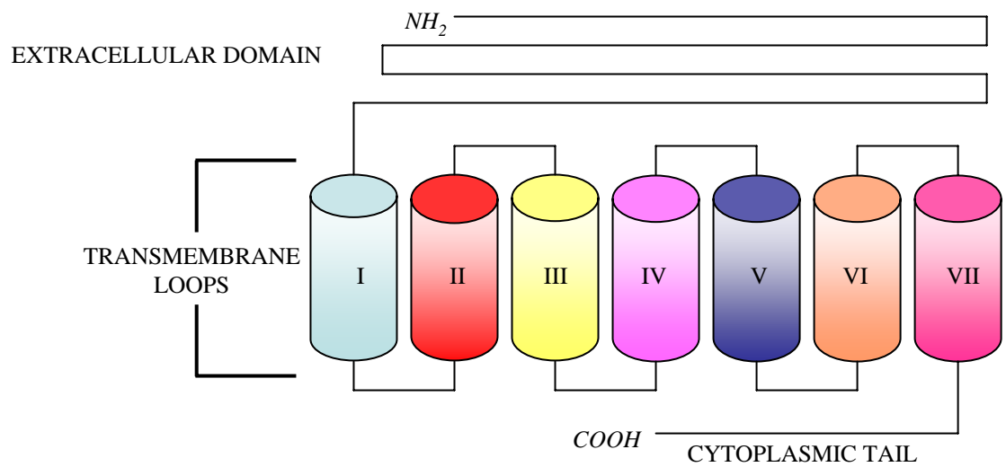
Figure 2-27. General topography of gonadotropin receptors.
