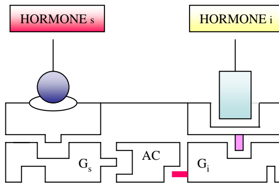
Figure 2-32. Competitive stimulatory and inhibitory transducer G proteins in hormonal regulation of adenyl cyclase.
