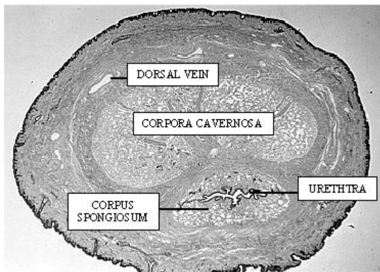
Figure 3-14. Photomicrograph of a cross-section of human vascular penis.
