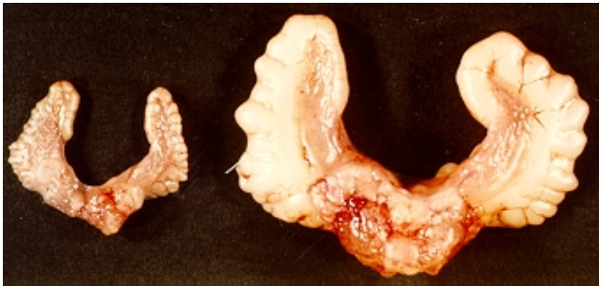
Figure 3-16. Effect of castration (left) on rat seminal vesicles. Glands from a sham- operated control are shown on the right.
