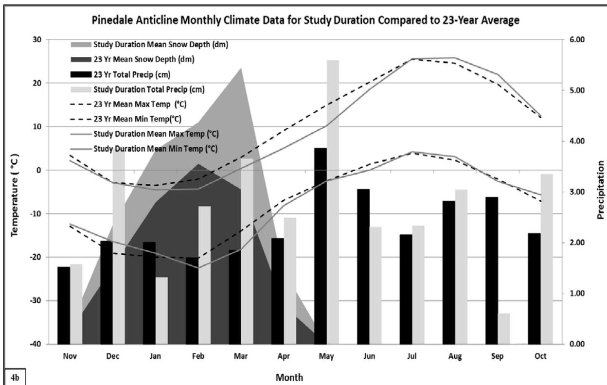
Figure 4a. Monthly climate data for study duration and 23 year average for the Jonah Field study site and 4b. the Pinedale Anticline study site (Western Regional Climate Center, 2012).
