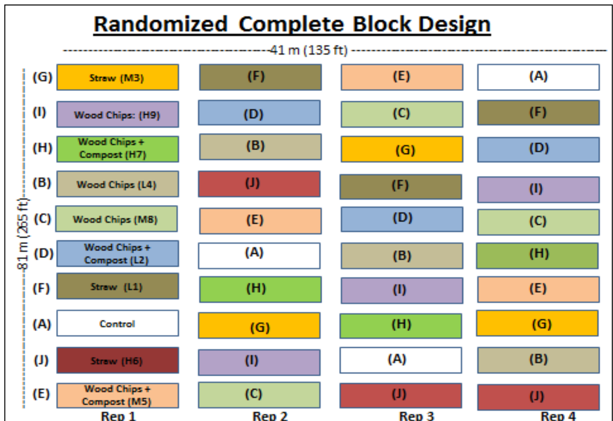
Figure 5. Field plot layout.
