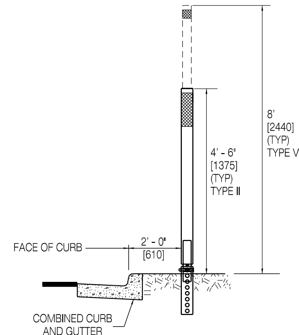
TYPICAL PLACEMENT-RURAL SECTIONS WITH CURB & GUTTER W/O SIDEWALK
